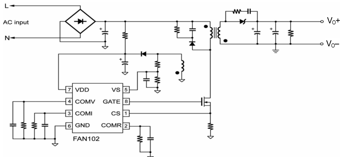
Figure 2. Typical Application
