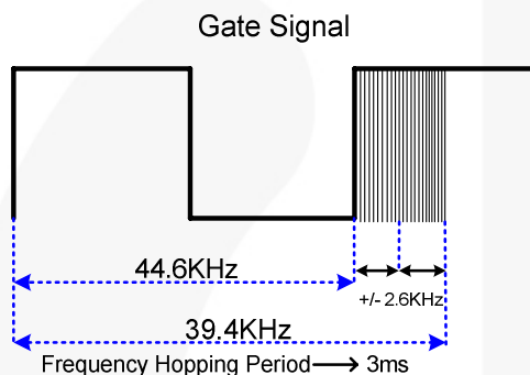
Figure 24. Frequency Hopping
