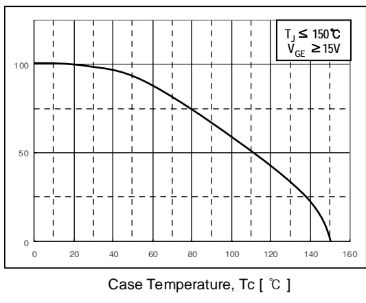
Fig 12. rated Current vs. Case Temperature
