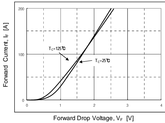
Fig 15. Forward characteristics
