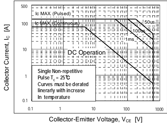
Fig14. SOA characteristics
