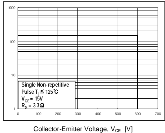
Fig 10. RBSOA Characteristic
