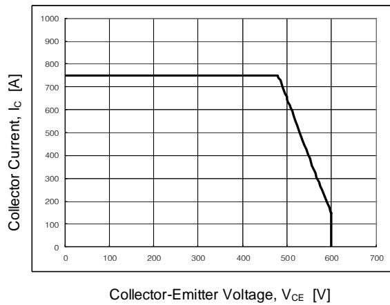
Fig 11. SCSOA Characteristic
