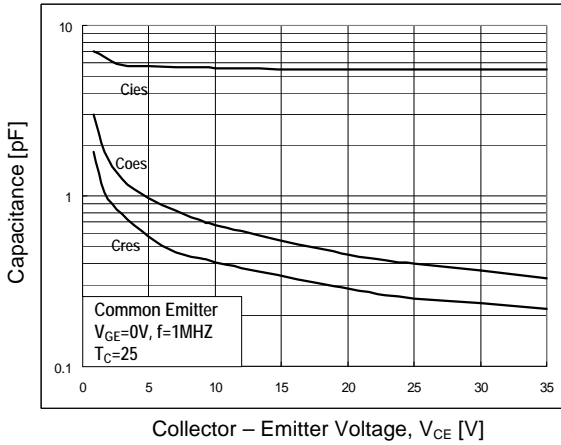
Fig 7. Capacitance characteristics
