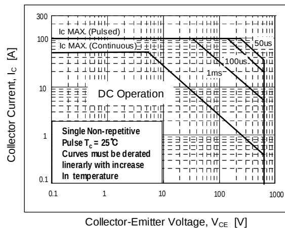
Fig14. SOA characteristics
