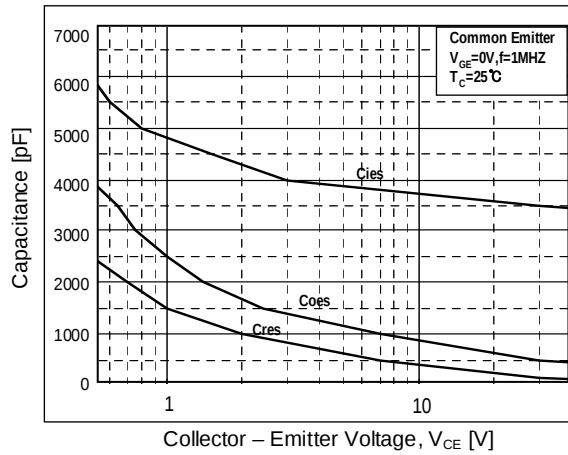
Fig 7. Capacitance characteristics
