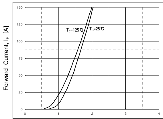
Forward Drop Voltage, V_F [V] Fig 10. Forward characteristics
