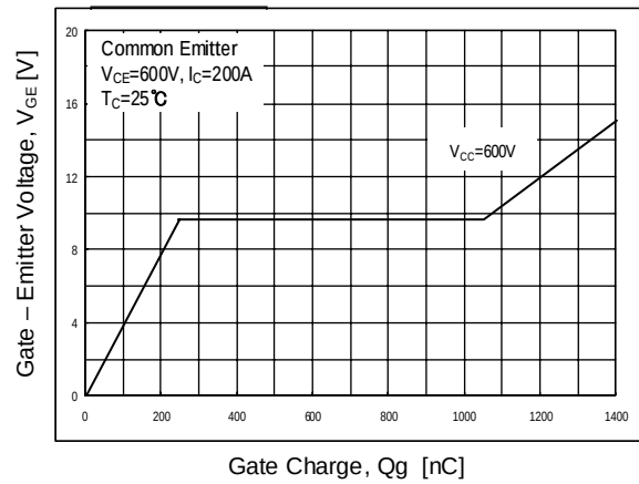
Fig 8. Gate Charge characteristics
