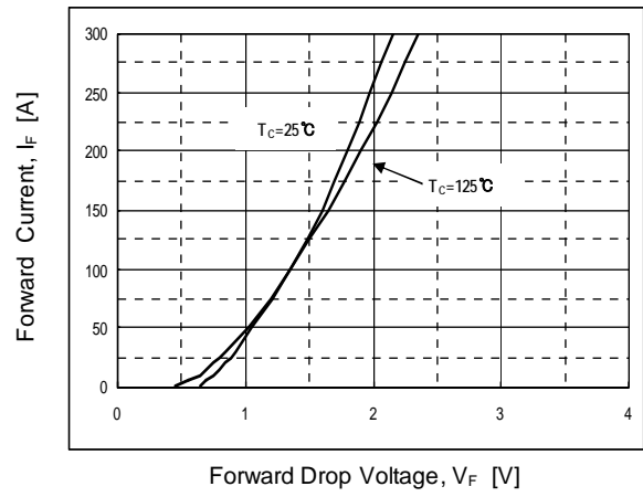
Fig 14. Forward characteristics
