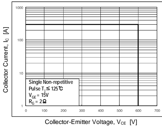
Fig 9. RBSOA Characteristic
