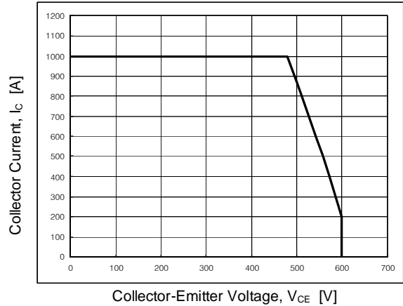
Fig 10. SCSOA Characteristic
