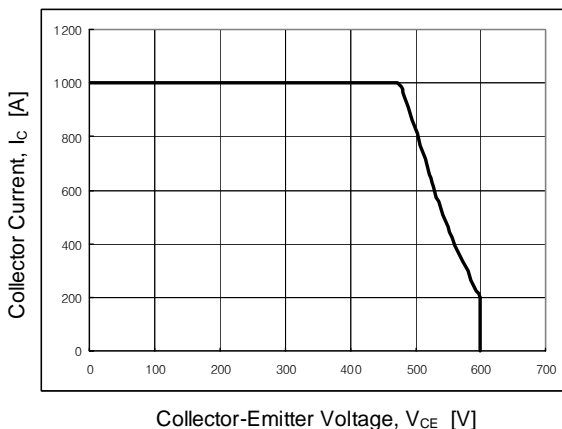
Fig 11. SCSOA Characteristic
