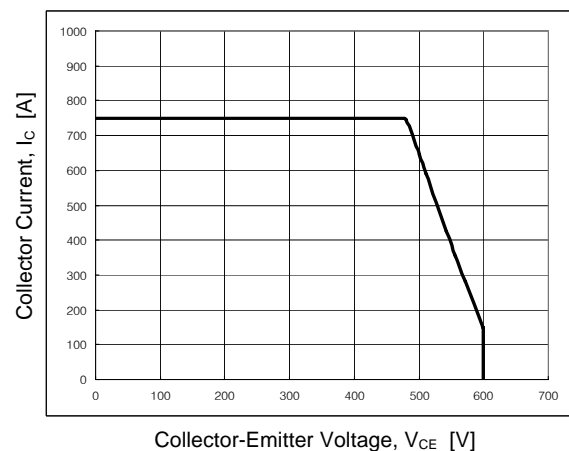
Fig 12. SCSOA Characteristic
