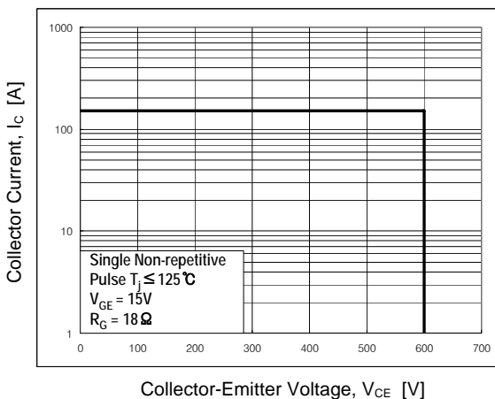
Fig 11. RBSOA Characteristic
