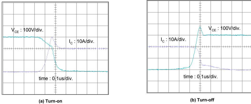
Fig. 5. Experimental Results of Switching Waveforms Test Condition: V_{dc}=300V , V_{cc}=15V , L=500\mu H (Inductive Load), T_C=25^\circ C
