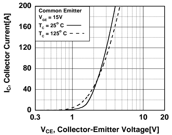
Fig 2. Typical Saturation Voltage Characteristics
