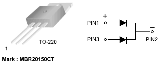
Mark : MBR20150CT
