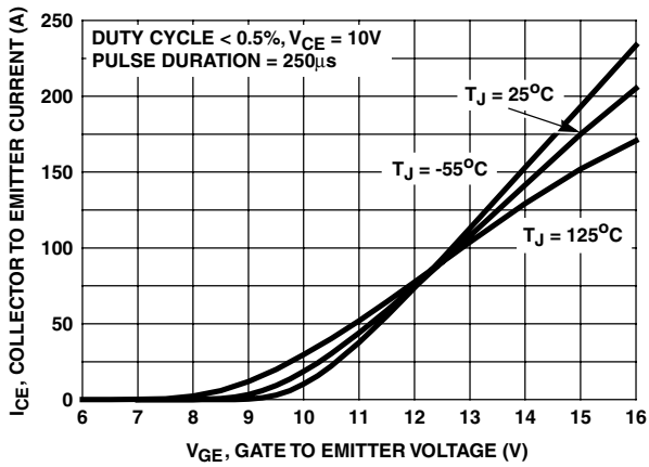
FIGURE 13. TRANSFER CHARACTERISTIC
